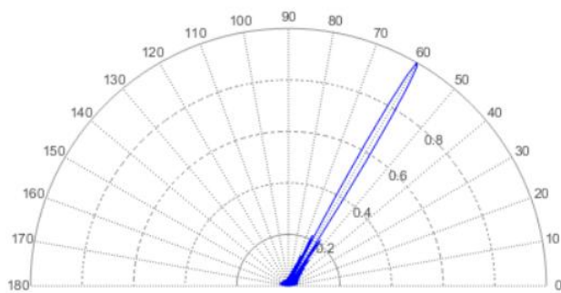
Radiation Pattern for N=40, Beamwidth ~ 5°
